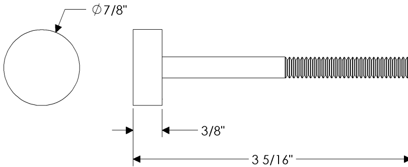
TBCAP1 Thru-Bolt Screw Cap 7/8" Diameter
