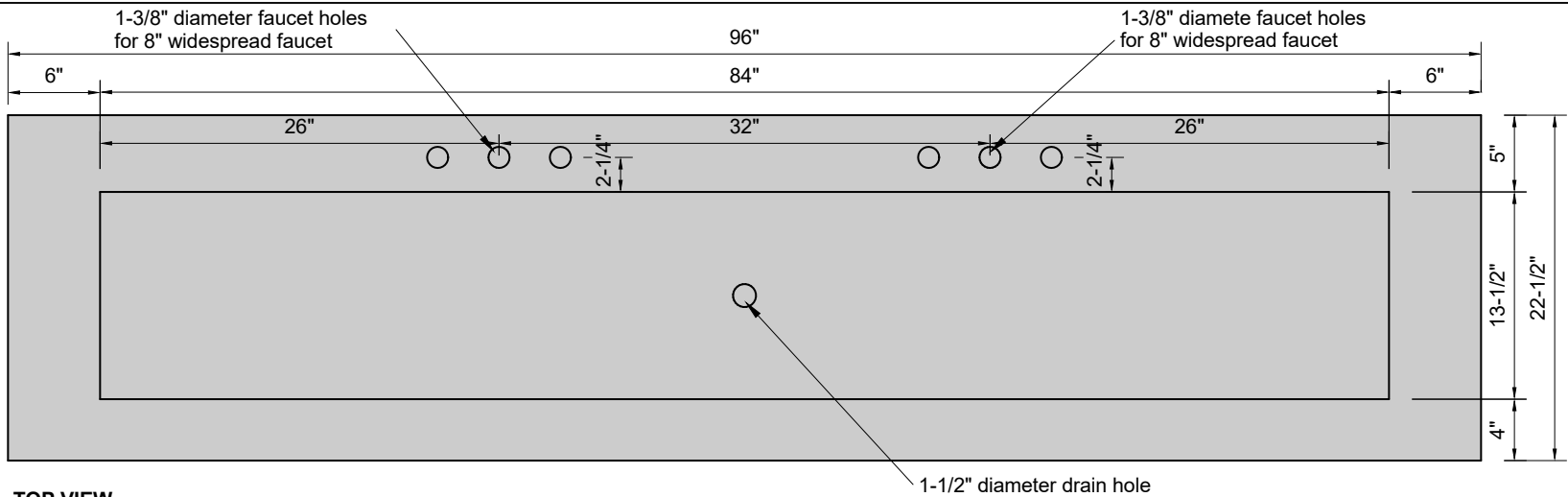
TOP VIEW
