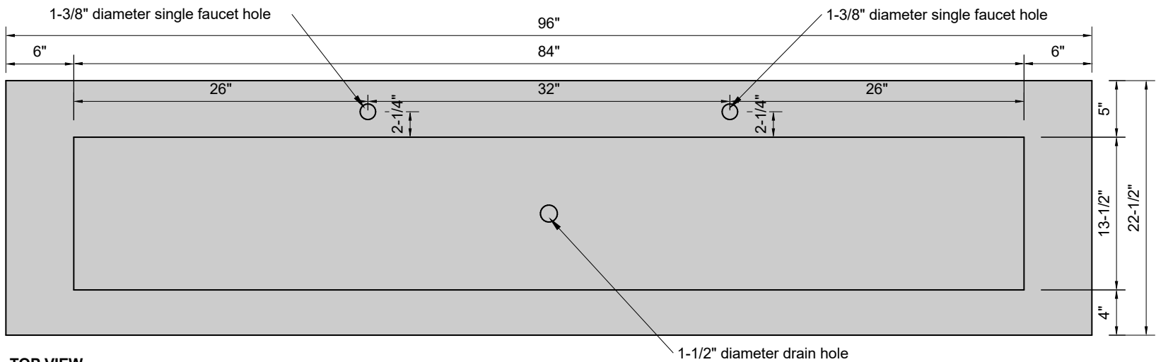
TOP VIEW
