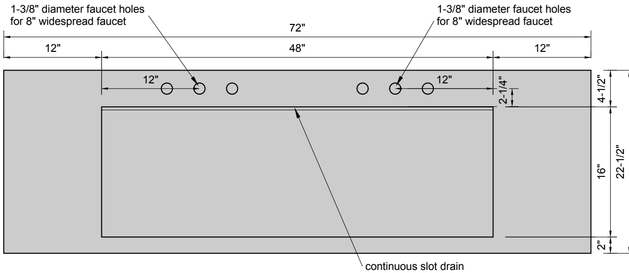
PLAN VIEW
